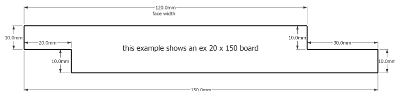
Example: vertical half lap rebate
